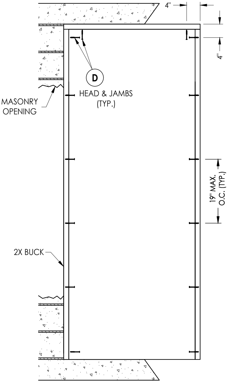
BUCK ANCHORING
